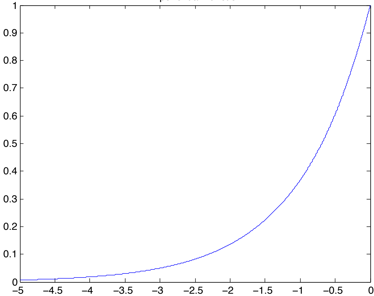
Exponential Function
